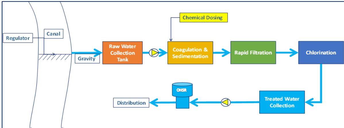
Figure 1: Schematic design of Water Network Investments
